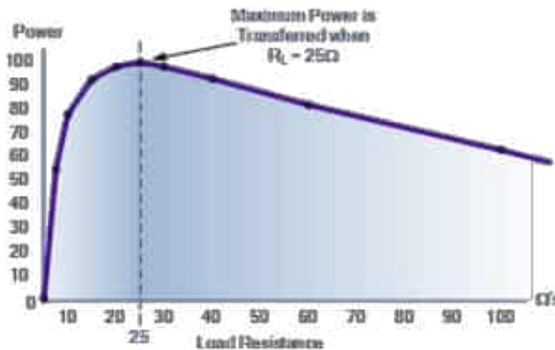
Fig:10.7 Maximum Power transfer
