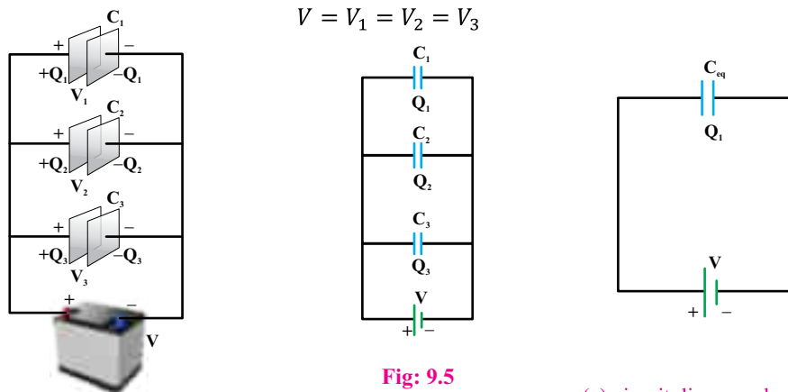
(a) a pictorial representation of three capacitors connected in parallel to a battery
