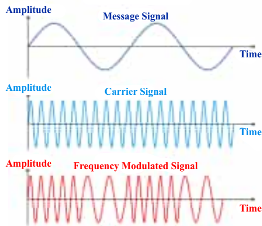
Fig: 14.11 Frequency Modulation
