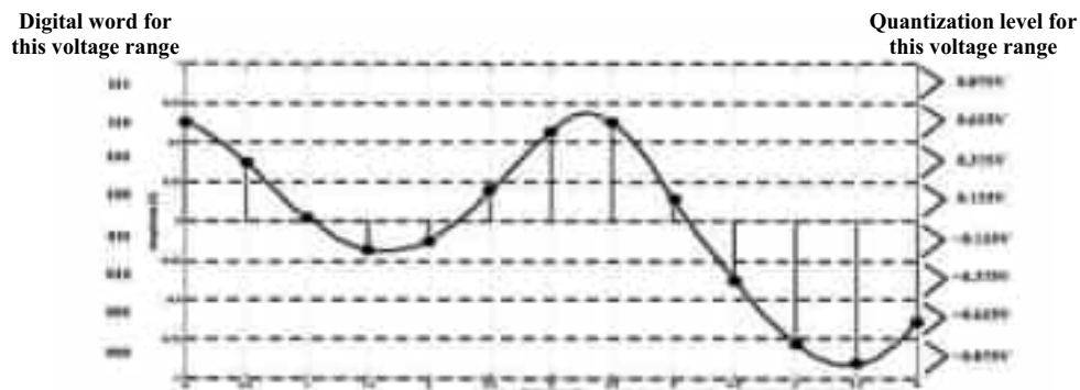
Fig. 14.17 Coding Waveform
