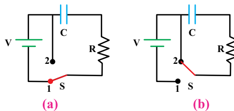
Fig: 9.7 Resistor Capacitor (RC) circuit.
