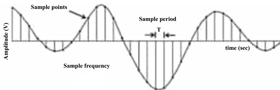
Fig: 14.16 Sampling Waveform
