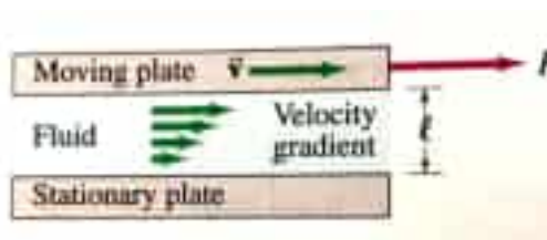
Fig: 7.1 viscous fluid between two plates
