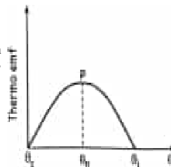
Fig:10.9 Variation of thermoelectric emf
