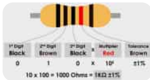
Resistance of 5 Band Resistor
