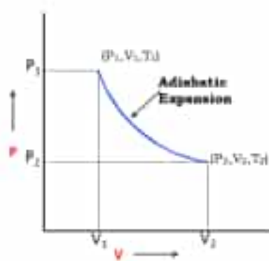
Fig: 12.3 An adiabatic behavior of gas
