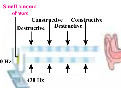
Fig: 12.8 The ear identify the amplitude (intensity) cycling from large to small then small to large and then large to small as pulsation in loudness. Thus, we refer this phenomenon of beats as interference of sound waves in time.
