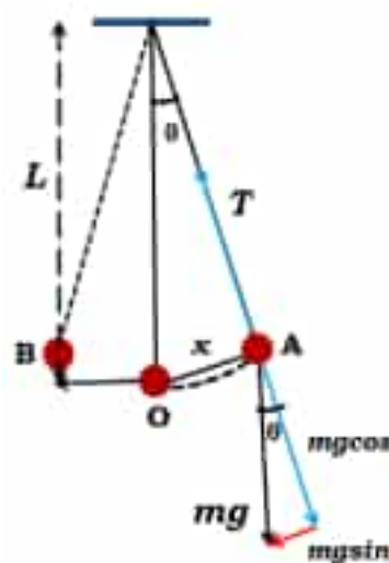
Fig. 11.14 Motion of simple pendulum.
