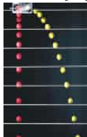
Projectile Motion Fig: 2.25
