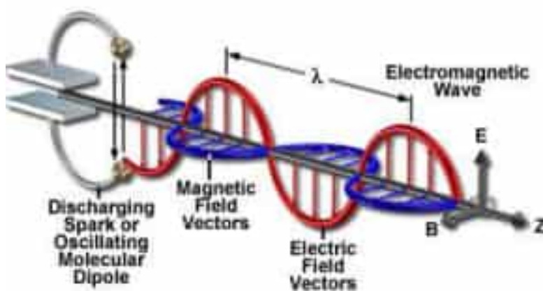
Fig: 13.3 Propagation of electromagnetic waves.
