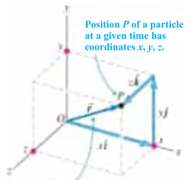
Position vector of point P has components x, y, z.
