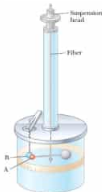
Fig: 8.1 Coulomb's torsion balance.
