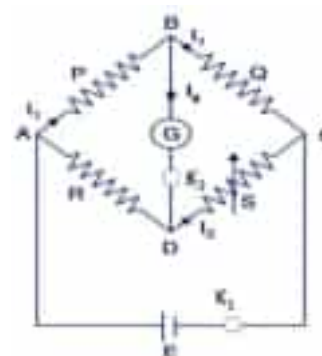
Fig: 10.17 Wheatstone Bridge
