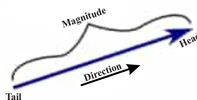
Fig: 2.1 Representation of vector
