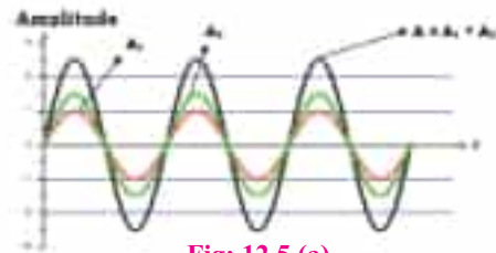
Fig: 12.5 (a) Two coherent waves with phase difference \varphi (Red and Green) showing constructive interference. Destructive Interference
