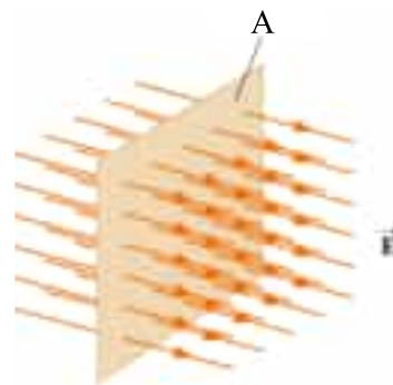
Fig: 8.9 The field lines penetrating through a rectangular surface of area.
