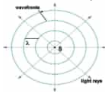
Fig: 13.11 Circular wave fronts
