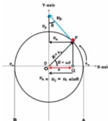
Fig: 11.10 velocity of projection
