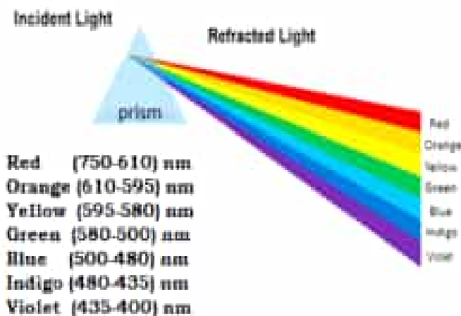
Fig: 13.9 Dispersion of white light through a prism.
