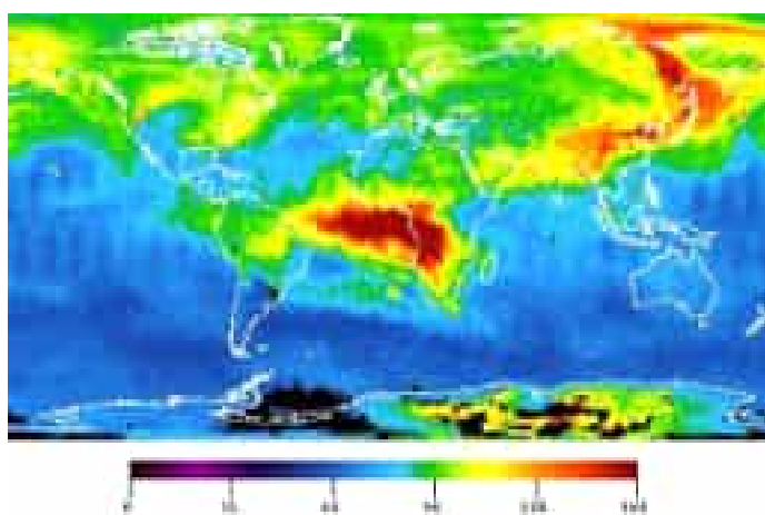
Fig: 13.6 An image of Earth in infrared wavelengths shows relative temperatures in Fahrenheit around the world.
