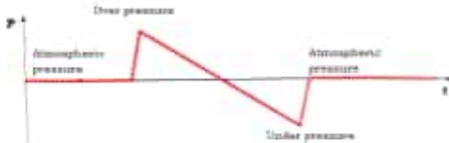
Fig: 12.25 The variation in pressure at a point on the ground as a supersonic plane flies overhead.
