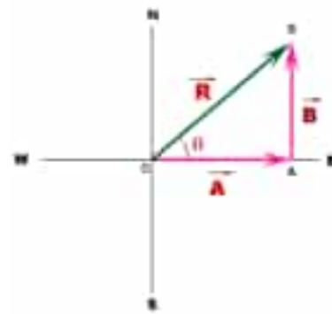
Fig: 2.2 Addition of vectors A and B
