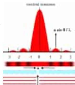
Fig: 13.26 Single slit diffraction. The intensity of light is gradually decreasing from right and left of central maxima
