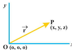
Fig: 2.9 position vector
