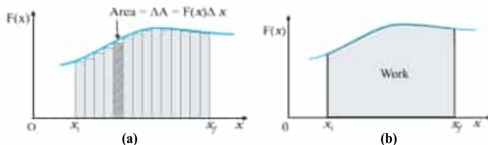
Fig: 5.6 (a and b) variable force displacement graph
