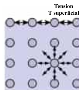
Fig: 6.7 Surface tension
