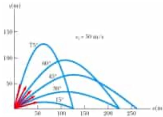
Fig: 2.27 range covered at different angles
