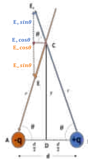
Fig: 8.8 Electric dipole formed by two charges +q and -q .
