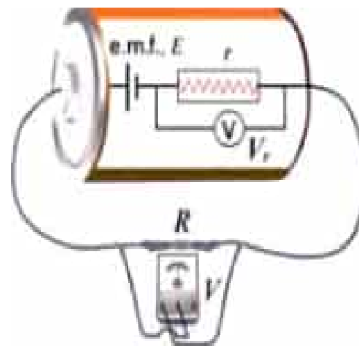
Fig:10.4 Internal resistance of a source
