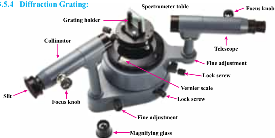
Figure.13.28. A Diffracting spectroscope
