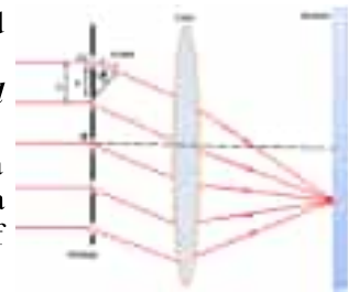
Fig: 13.29 Geometrical illustration of a diffraction grating.
