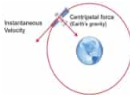
Fig: 4.10 Orbital velocity of satellite
