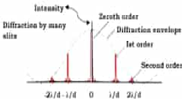
Fig: 13.30 Multiple slits sharp energy spectrum maxima.
