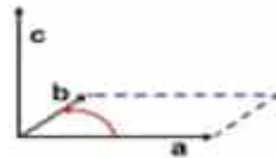
Fig:2.17 cross product of A \times B
