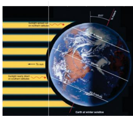
Figure 10.8 Earth at Winter Solstice
