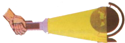
Figure 10.4 Demonstration of Day and Night
